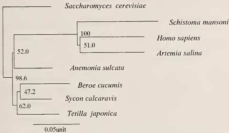
FIG. 2. Phylogenetic relationships of diploblasts with triploblasts ( Schistosoma mansonii , Artemia salina , and Homo sapiens ) as deduced by reference to yeast as the out group. The tree was constructed by neighbor-joining. The scale bar indicates an evolutionary distance of 0.05 nucleotide substitutions per sequence position. Numbers at each branch indicate the percentage of times a node was supported in 500 bootstrap pseudoreplications by neighbor-joining. The ctenophore Beroe forms a unit with poriferans.
